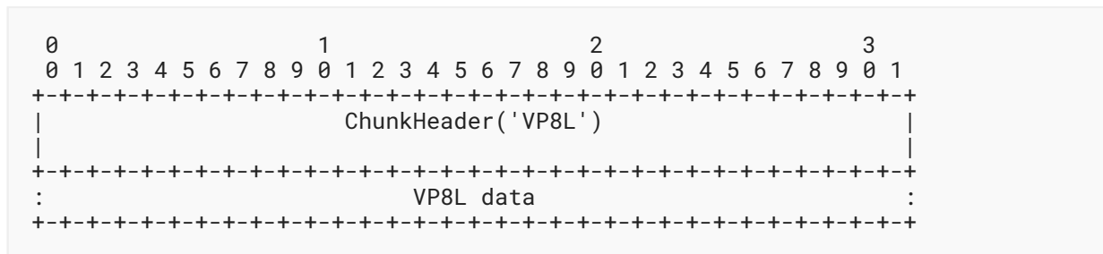
Figure 6: 'VP8L' Chunk
