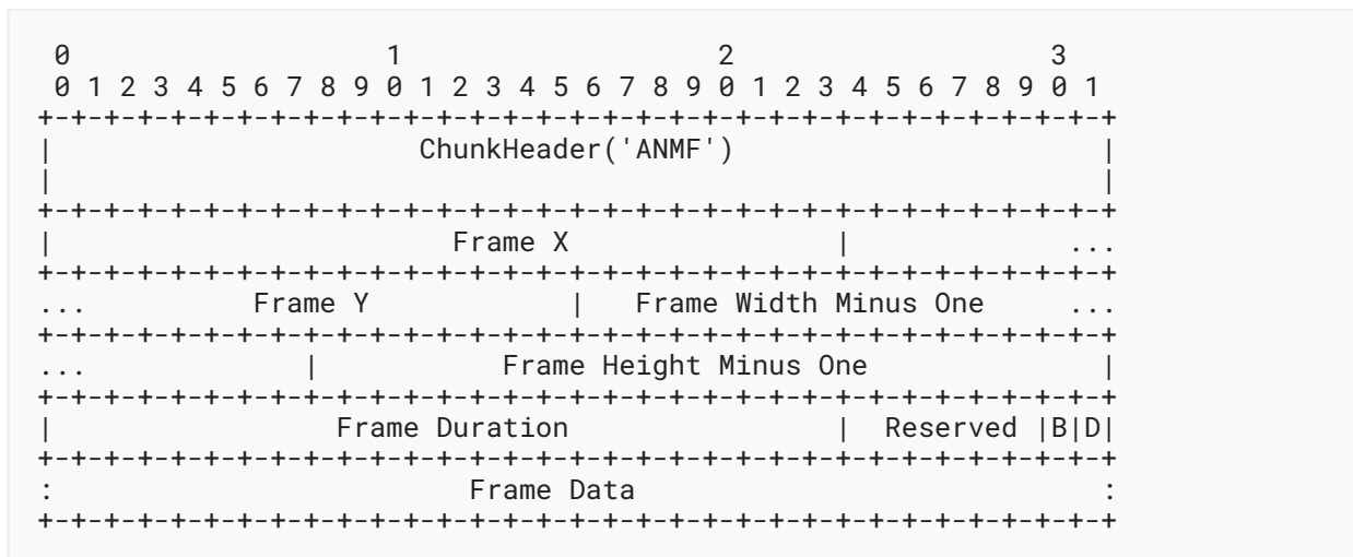
Figure 9: 'ANMF' Chunk
